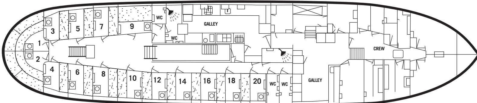
MAIN DECK
